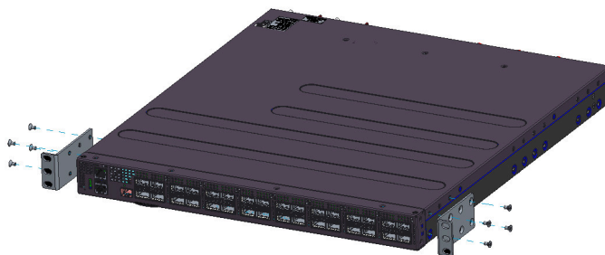
Figure 2.2. Front brackets installation
