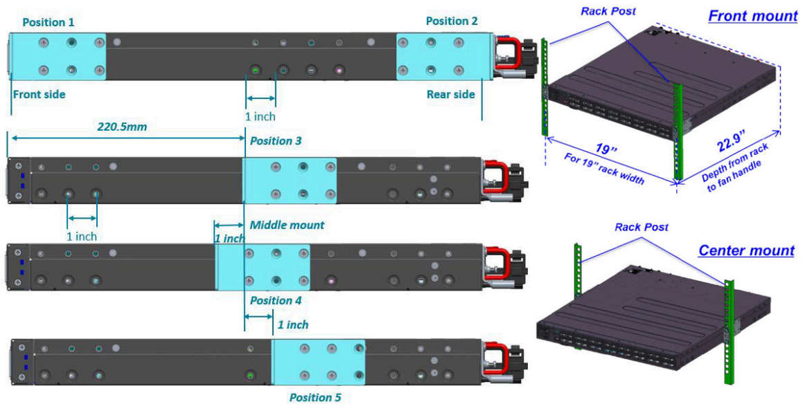
Figure 2.3. Mounting point options
