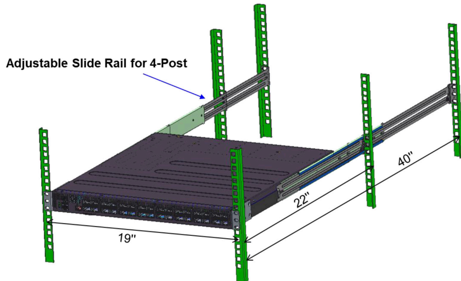
Figure 2.5. Mounting the switch
