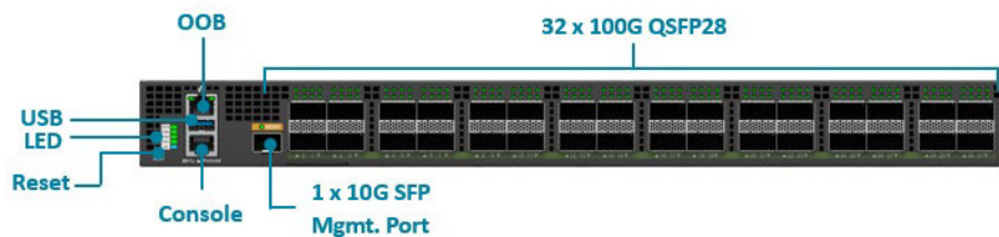
Figure 3.1. Aurora 721 front view
