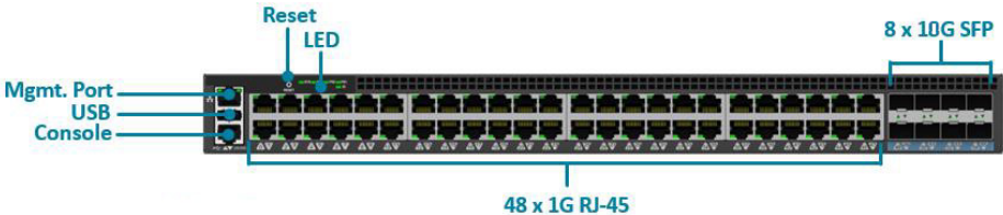
Figure 3.1. Aurora 221 front view
