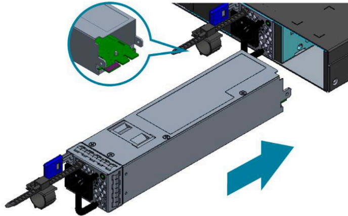
Figure 2.6. Inserting the PSU module
