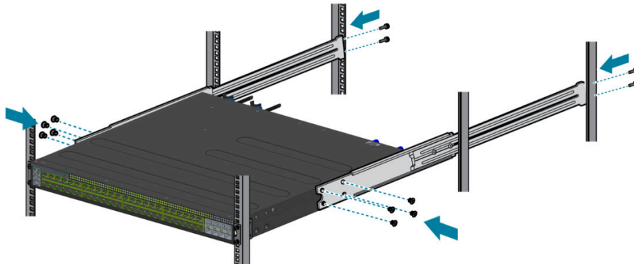
Figure 2.4. Mounting the switch
