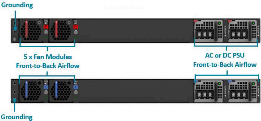
Figure 3.2. Aurora 221 rear view
