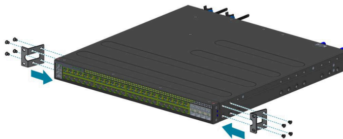
Figure 2.1. Front brackets installation
