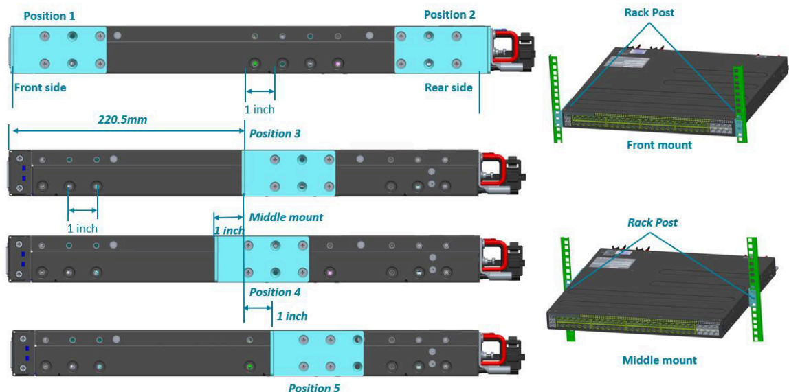
Figure 2.2. Mounting point options
