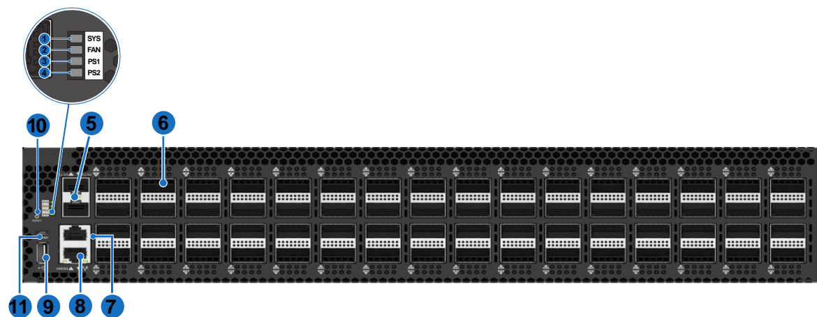
Figure 3.1. Aurora 750 front view
